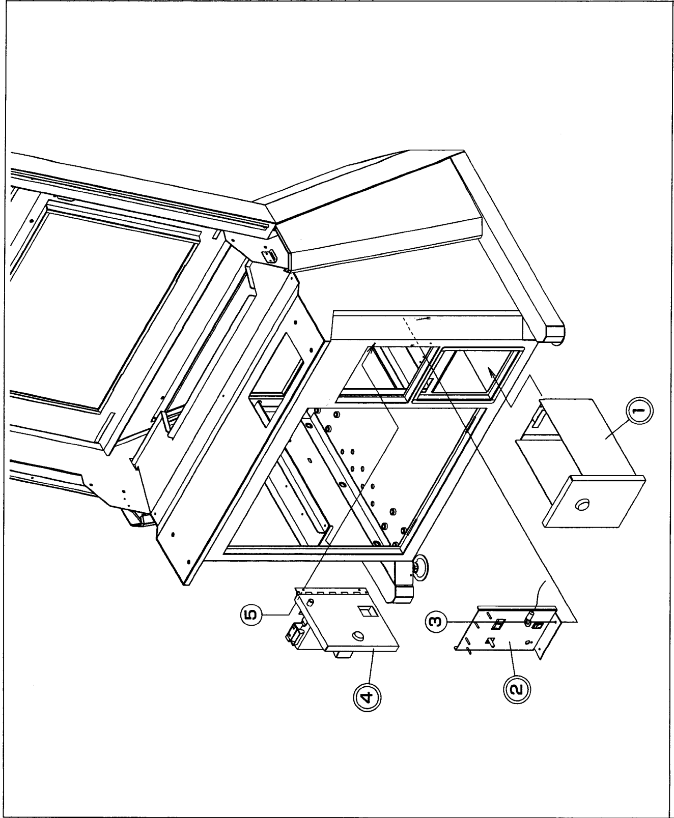
CABINET ASSY [6]
