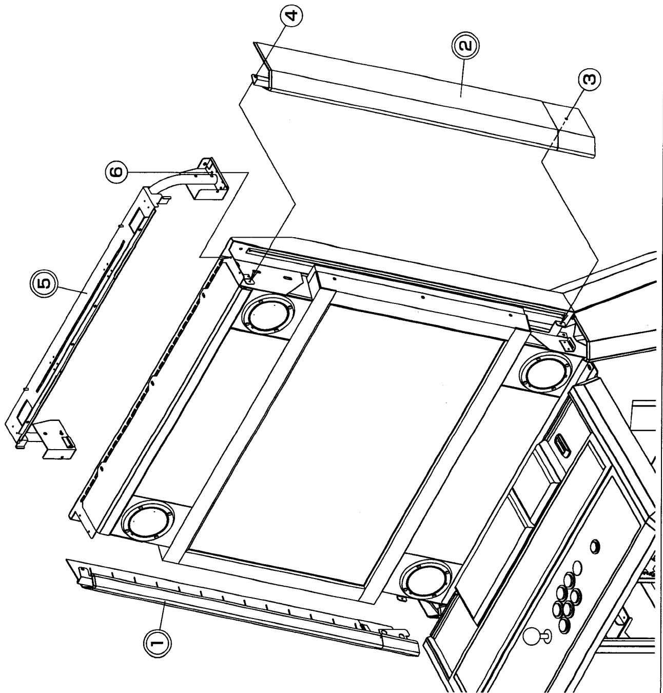
CABINET ASSY [10]
