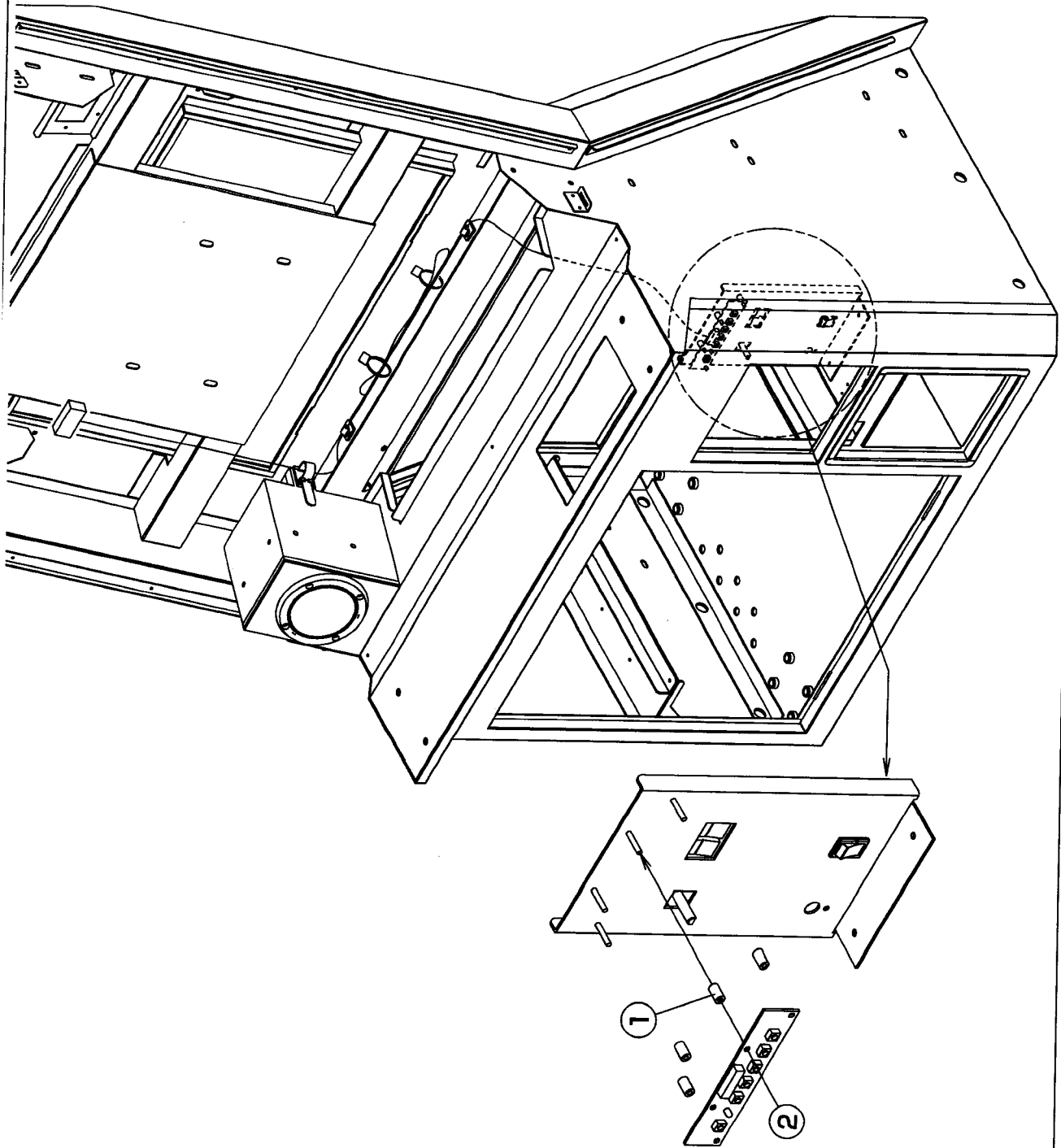
CABINET ASSY-(MAIN) [1]
