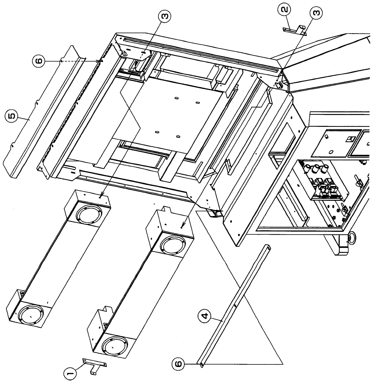
CABINET ASSY [8]
