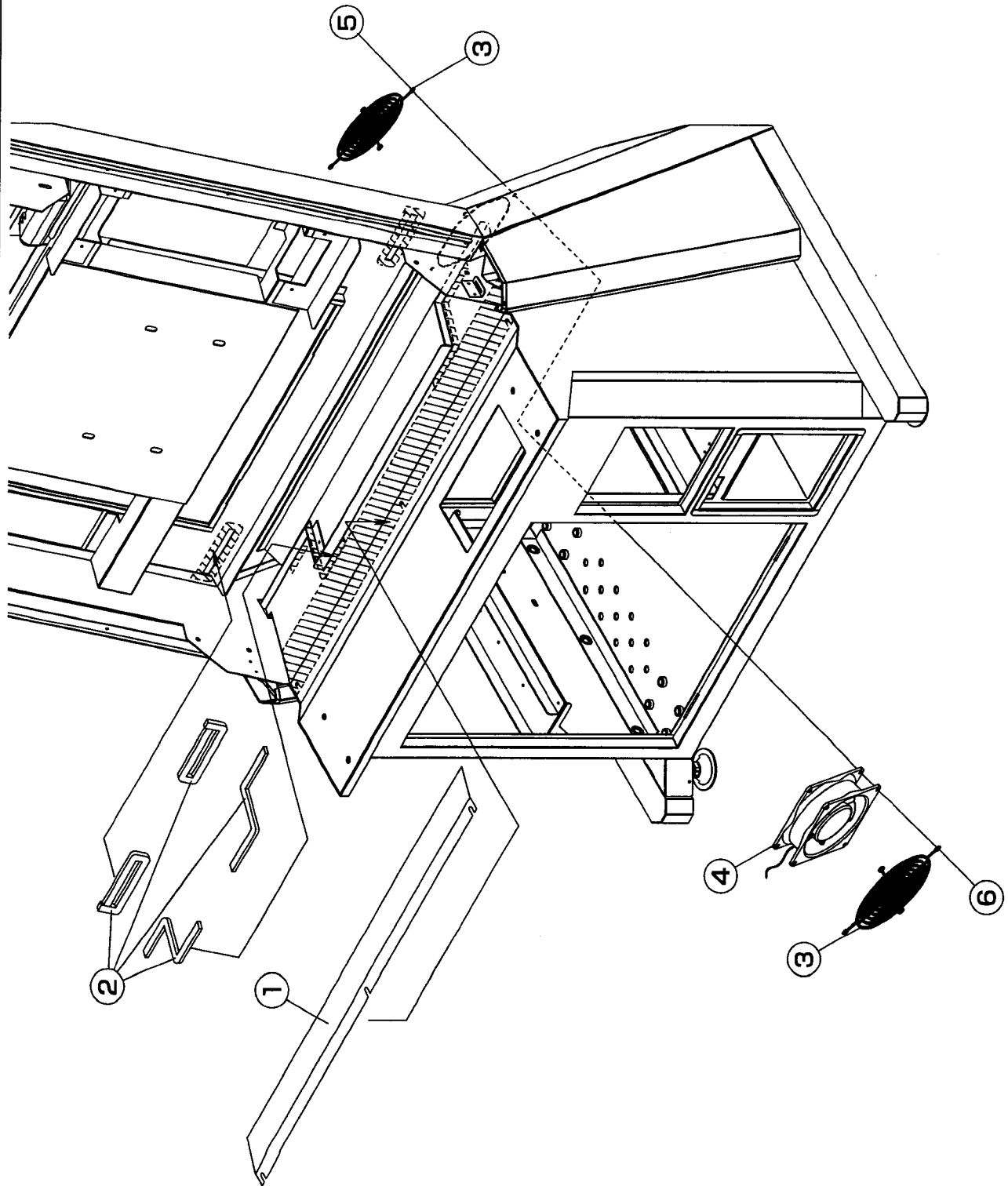
CABINET ASSY [4]
