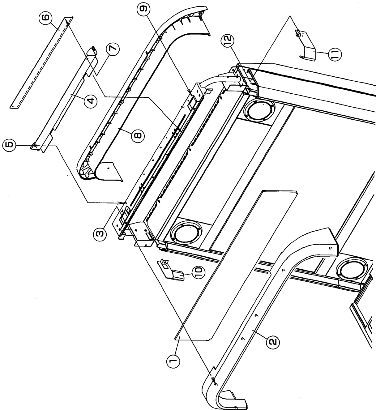
CABINET ASSY [11]
