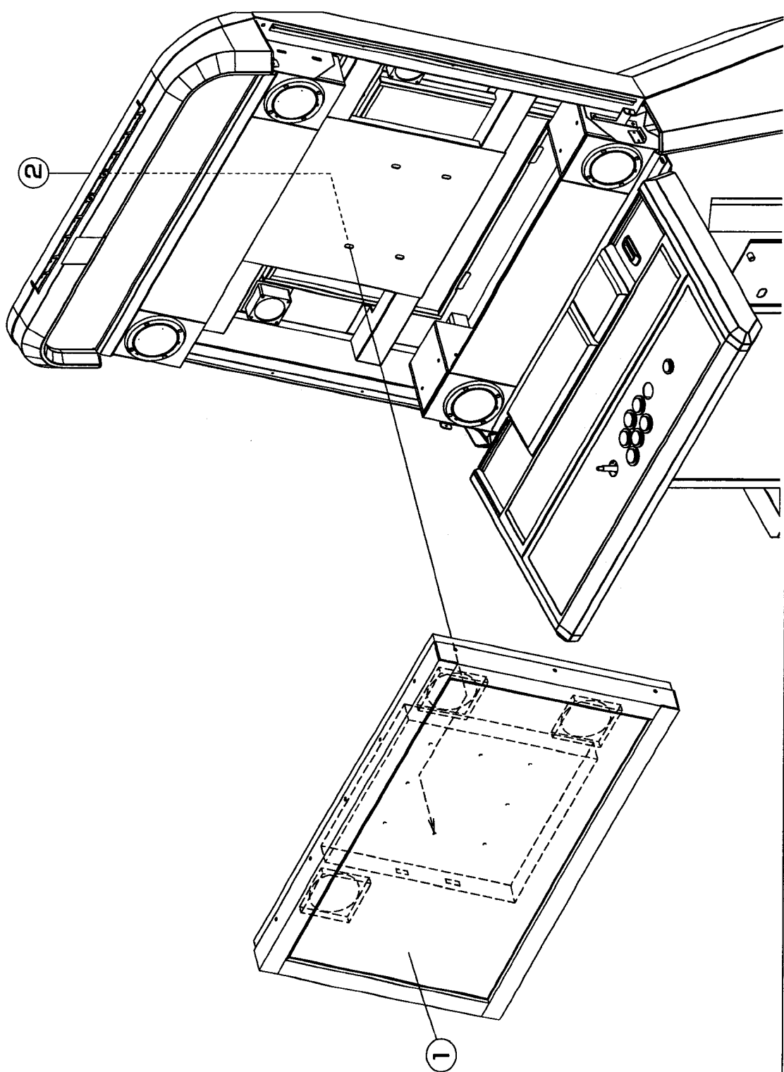
CABINET ASSY-(MAIN) [2]
